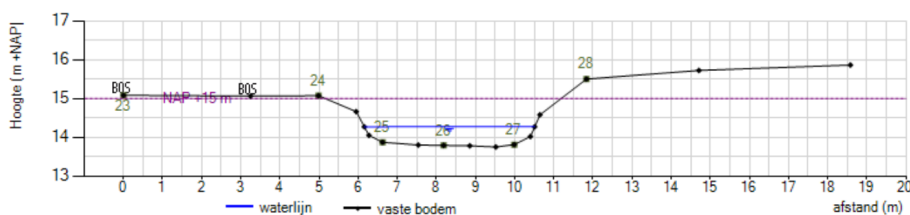
Figure 14: A cross-section of the Goorloop (234001P1390) at place of measuring point oGOORLO420 determined on the 22 nd of March 2012 showing that the width ( w_E ) is approximately 4.25 m, the depth ( d_E ) is approximately 0.5 m and the cross-section surface fraction ( f_{ca} ) about 0.9 [–].
